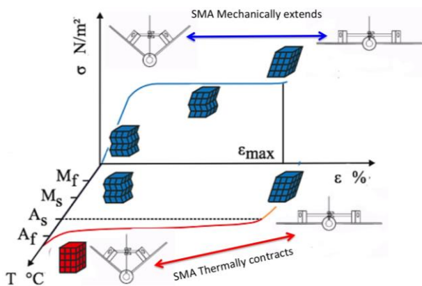
Fig. 6. Thermo-mechanical transformations of SMA adductor and abductor of the biomechanically inspired machine
