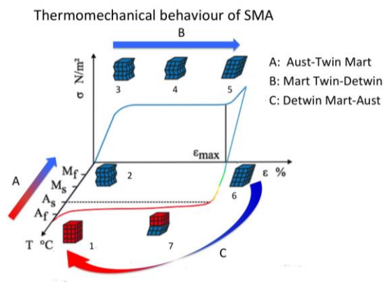
Fig. 1. SST diagram of thermal and mechanical induced transition in Shape Memory Alloys
