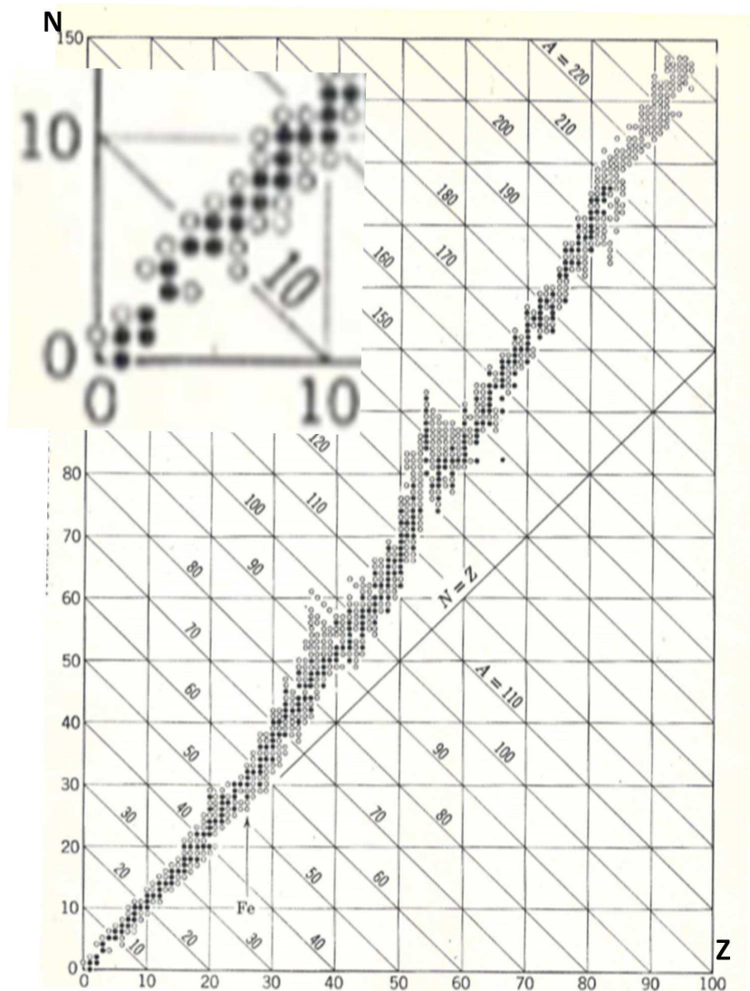
Fig. 1: Diagram of atomic cores (atomic nuclei). Source: (Halliday and Robert, 1966)
